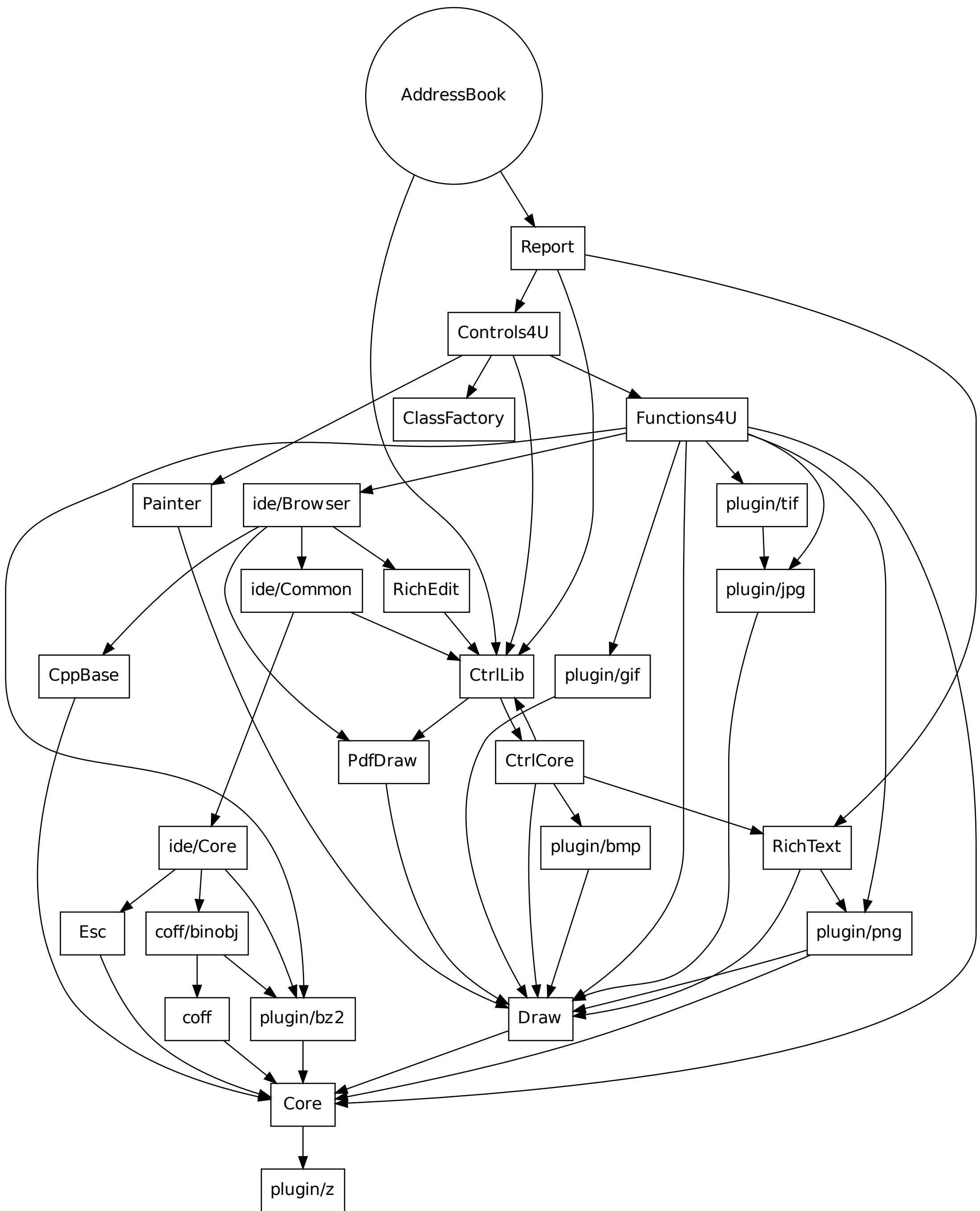
Package dependency graph of AddressBook
