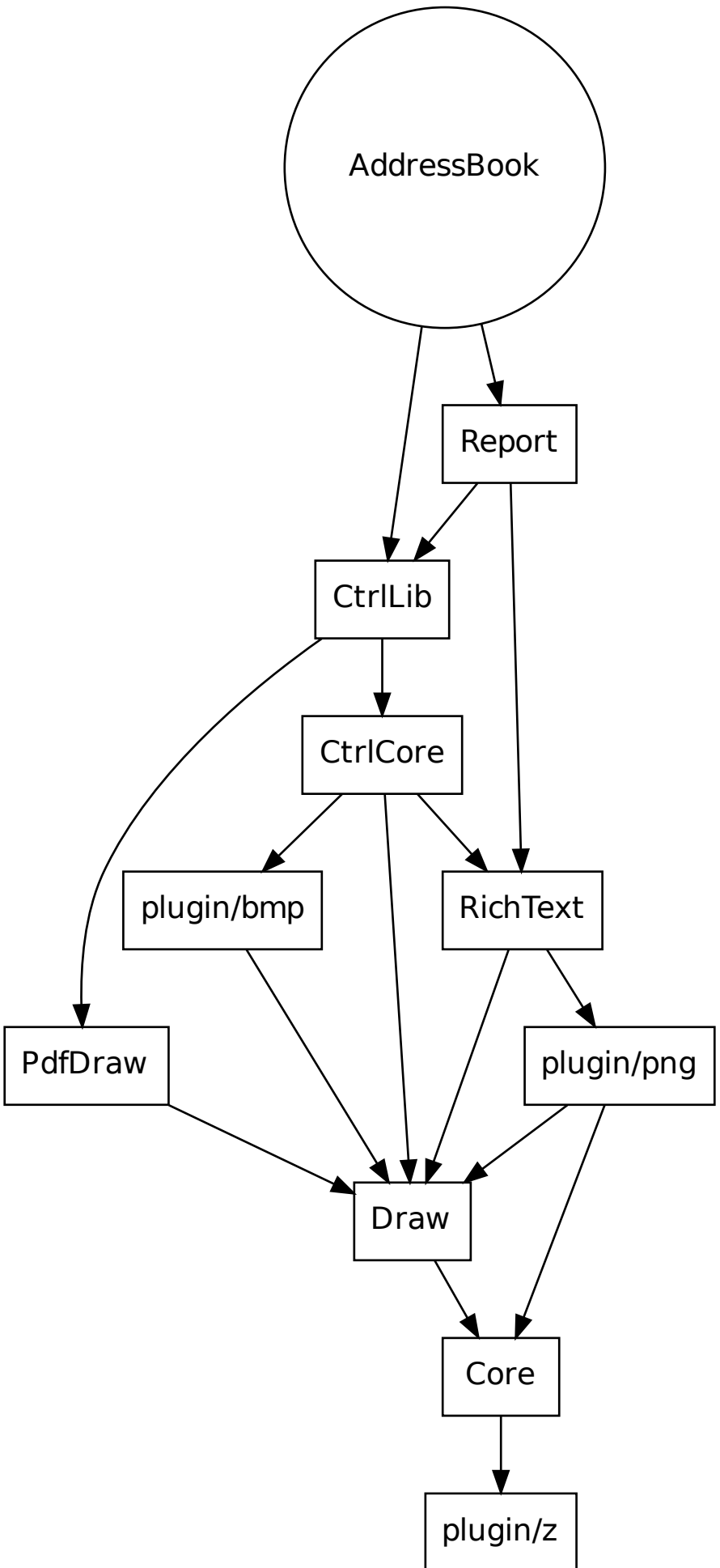
Package dependency graph of AddressBook
